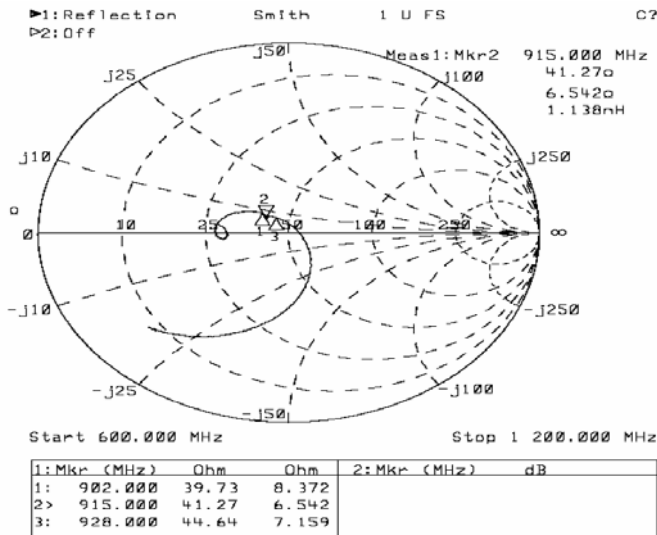
Figure 9. Input Impedance
