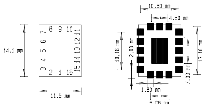
Figure 14. Recommended Land Pattern
