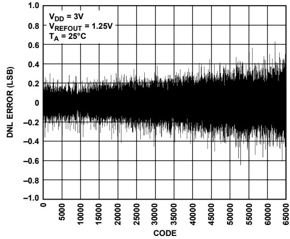
Figure 21. AD5667R DNL, 1.25 V Internal Reference
