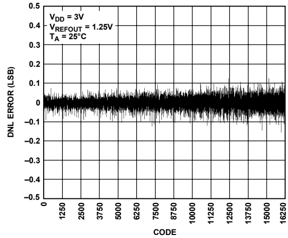
Figure 22. AD5647R DNL, 1.25 V Internal Reference
