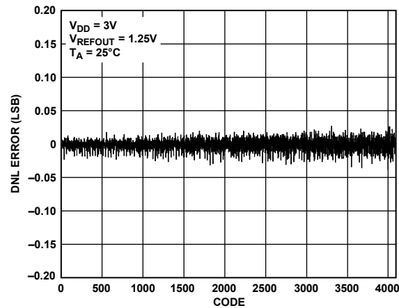
Figure 23. AD5627R DNL, 1.25 V Internal Reference
