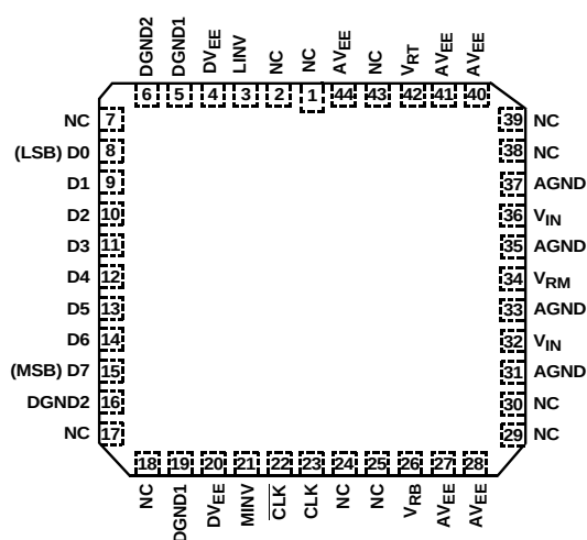
HI1386 (CLCC) TOP VIEW
