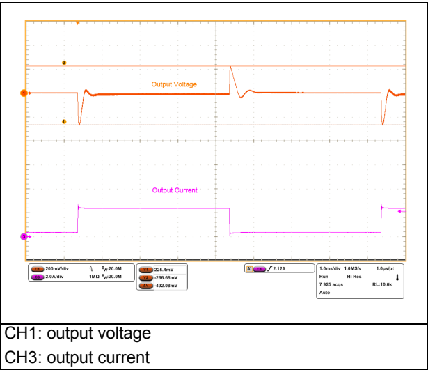
Figure 19. Dynamic load 2500 mA - 500 mA
