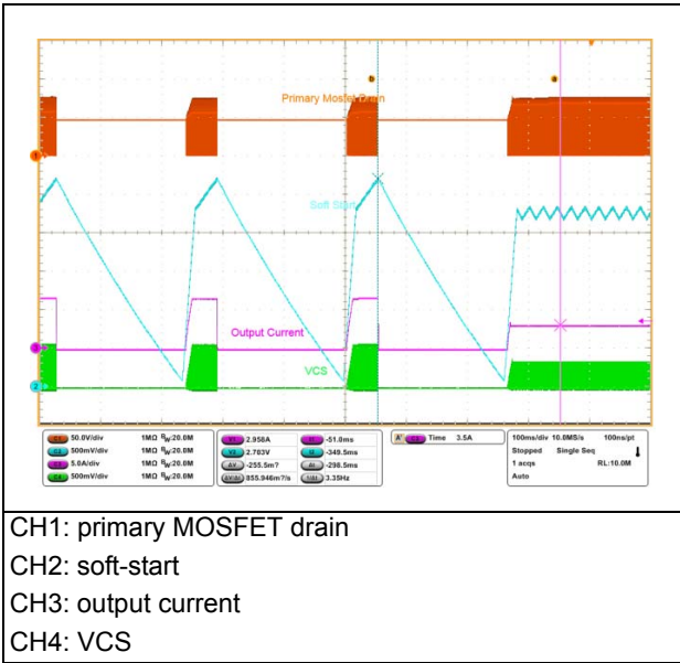
Figure 24. OCP removed - full load
