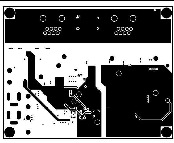
Figure 32. PCB layer: layer 2
