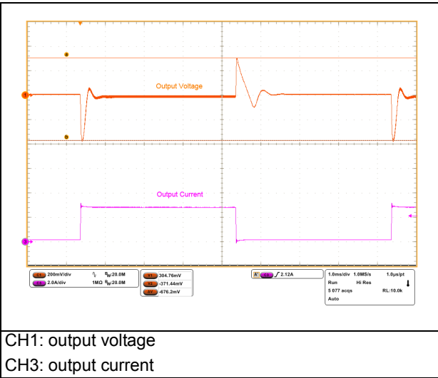
Figure 18. Dynamic load 3 A - 300 mA
