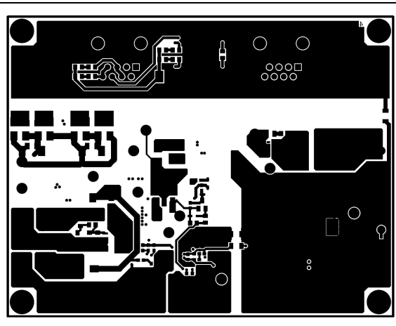
Figure 34. PCB layer: bottom view
