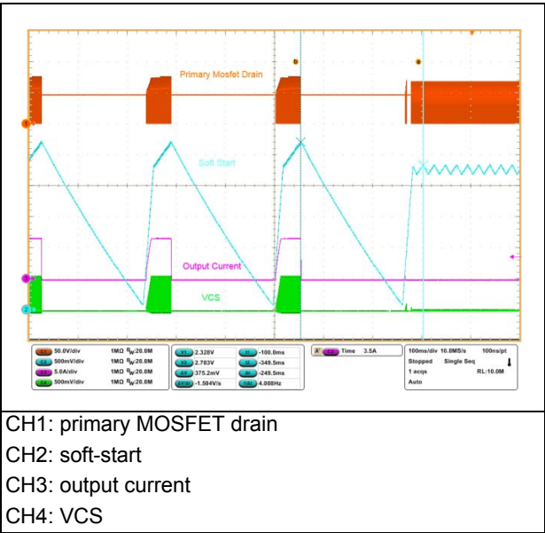
Figure 25. OCP removed - no load
