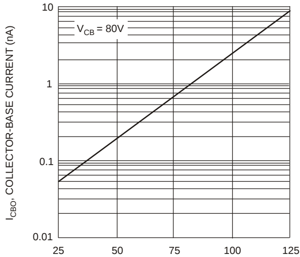
Fig. 5, Typical Collector-Cutoff Current vs. Ambient Temperature (DRDN005W)
