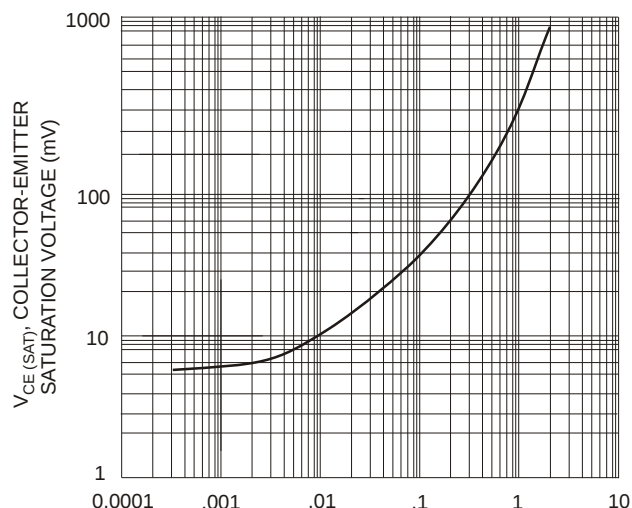
I_C , COLLECTOR CURRENT (A) Fig. 4, Collector Saturation Voltage vs. Collector Current (DRDN010W)
