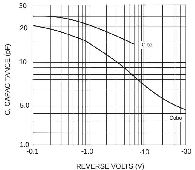
Fig. 16, Typical Capacitance (DRDP006W)
