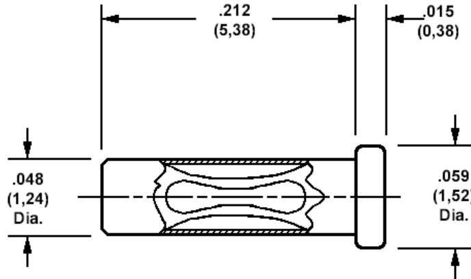
-01 - Closed bottom - Min hole depth .207 (5,26)
