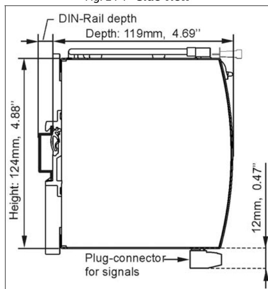
Fig. 24-1 Side view
