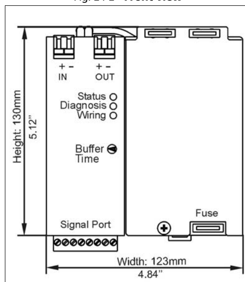
Fig. 24-2 Front view
