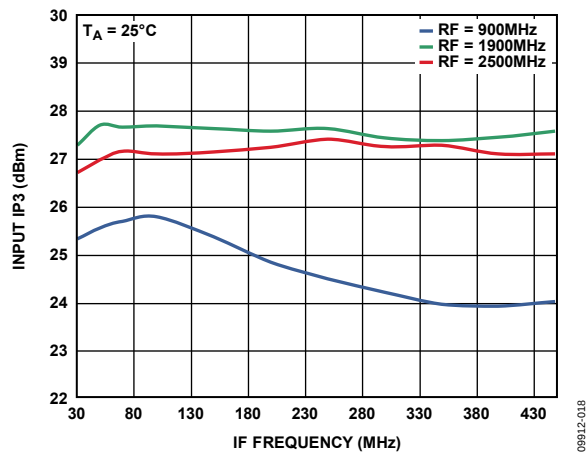
Figure 18. Input IP3 vs. IF Frequency
