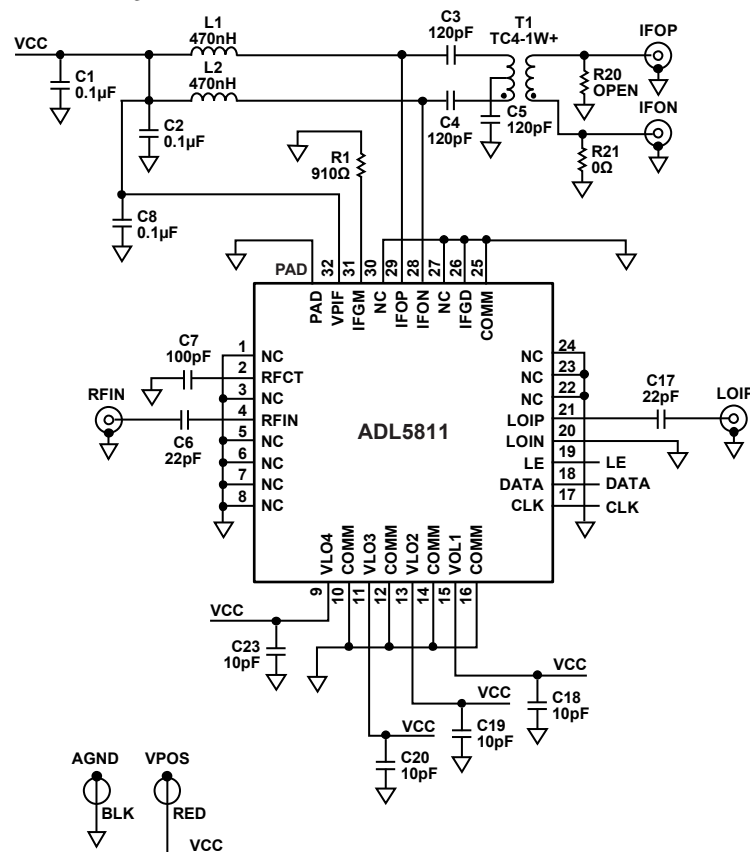
Figure 59. Basic Connections
