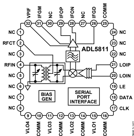
Figure 58. Block Diagram
