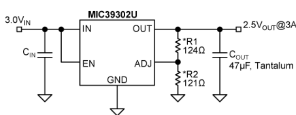
MIC39302 Adjustable Output Application
