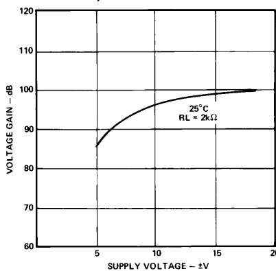
Figure 10. Open Loop Voltage Gain vs. Supply Voltage
