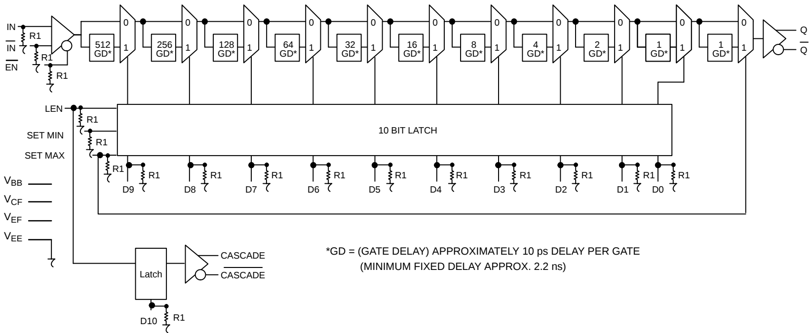
Figure 2. Logic Diagram
