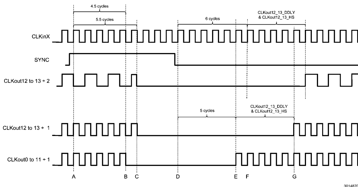
FIGURE 4. Clock Output synchronization using the SYNC1 pin (SYNC1 is Active Low, SYNC1_POL_INV=0) CLKout8_11_DIV = 1 CLKout12_13_DIV = 2 The digital delay for clock outputs 12 and 13 is 5 The digital delay half step for all clock outputs is 0 SYNC1_QUAL = 0 (No qualification) CLKout12_ADLY_SEL & CLKout13_ADLY_SEL is 0
