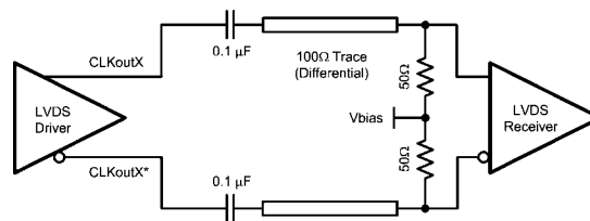
FIGURE 16. Differential LVDS Operation, AC Coupling, External Biasing at the Receiver
