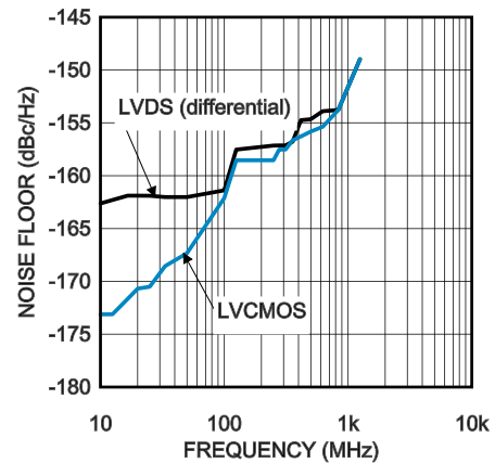
LVDS & LVC MOS Noise Floor vs. Frequency
