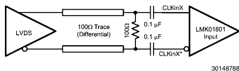
FIGURE 8. CLKInX/X* Termination for an LVDS Reference Clock Source
