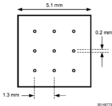
FIGURE 7. Recommended Land and Via Pattern
