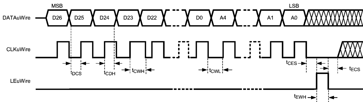
FIGURE 1. MICROWIRE Timing Diagram
