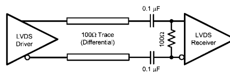
FIGURE 17. LVDS Termination for a Self-Biased Receiver
