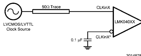
FIGURE 12. DC Coupled LVCMOS/LVTTL Reference Clock
