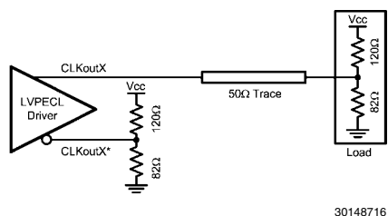
FIGURE 20. Single-Ended LVPECL Operation, DC Coupling, Thevenin Equivalent
