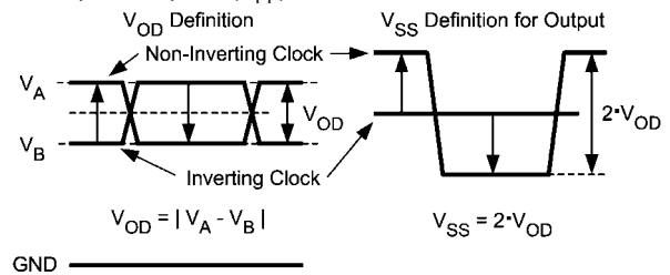
FIGURE 3. Two Different Definitions for Differential Output Signals
