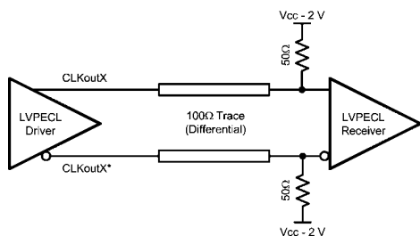
FIGURE 14. Differential LVPECL Operation, DC Coupling
