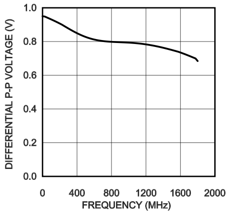
LVDS V_{SS} vs. Frequency (Note 19)
