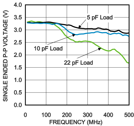
LVC MOS V_{pp} vs. Frequency
