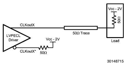
FIGURE 19. Single-Ended LVPECL Operation, DC Coupling
