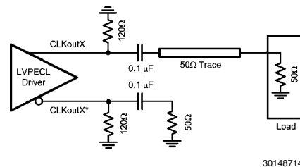
FIGURE 21. Single-Ended LVPECL Operation, AC Coupling R_{em}=120\ \Omega\ \text{to}\ 240\ \Omega
