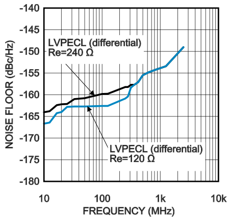
LVPECL Noise Floor vs. Frequency
