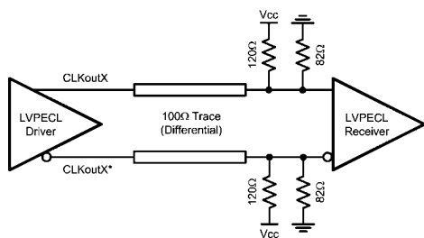
FIGURE 15. Differential LVPECL Operation, DC Coupling, Thevenin Equivalent
