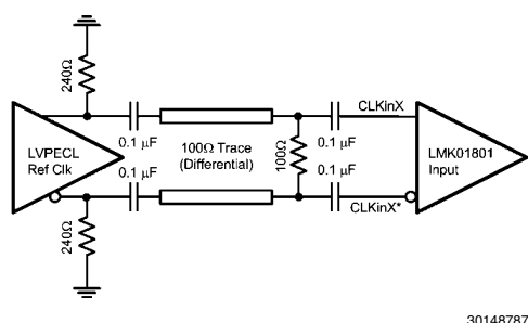
FIGURE 9. CLKInX/X* Termination for an LVPECL Reference Clock Source
