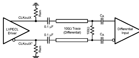
FIGURE 18. Differential LVPECL Operation, AC Coupling, External Biasing at the Receiver, R_{em} = 120\ \Omega to 240\ \Omega
