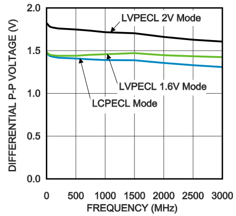
LVPECL V_{SS} vs. Frequency (Note 19)
