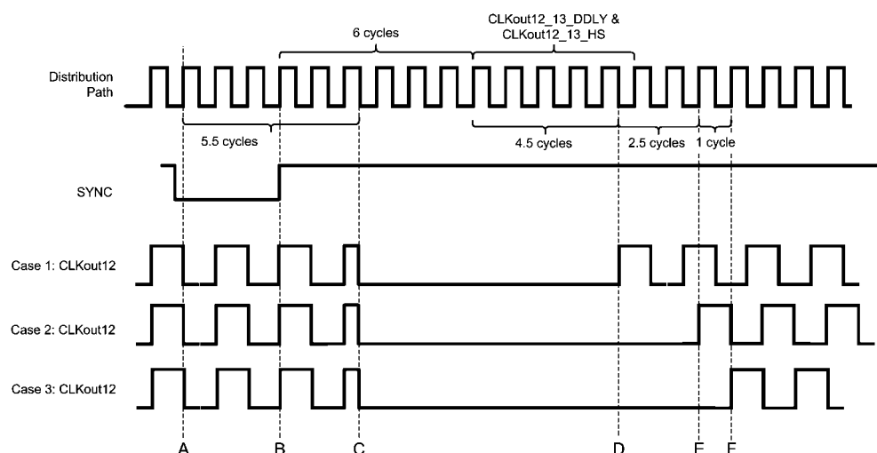
FIGURE 5. Clock Output synchronization using the SYNC pin (SYNC is Active Low, SYNC_POL_INV=1)
