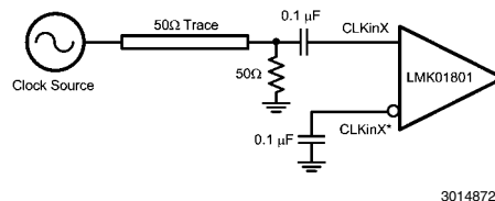
FIGURE 11. DC Coupled LVCMOS/LVTTL Reference Clock
