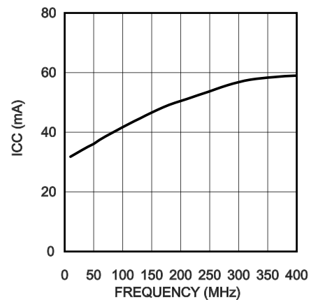
Typical Dynamic I_{CC} , C_L = 5\text{ pF}
