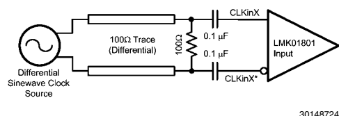
FIGURE 10. CLKInX/X* Single-ended Termination
