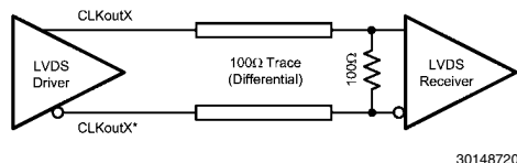
FIGURE 13. Differential LVDS Operation, DC Coupling, No Biasing of the Receiver
