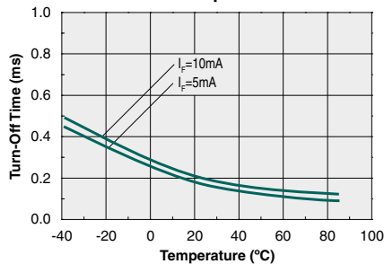
Typical Turn-Off Time vs. Temperature
