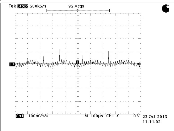
Figure 27. Output Ripple CH1 = V_{OCV} at Supply Output
