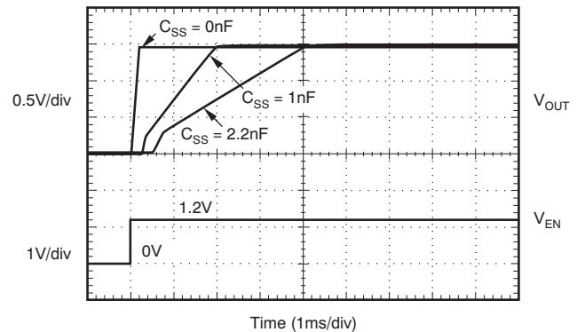
Figure 29. Turnon Response
