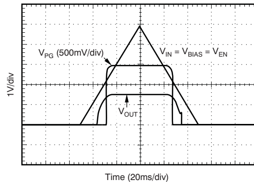
Figure 30. Power-Up/Power-Down
