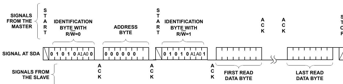
FIGURE 18. READ SEQUENCE
