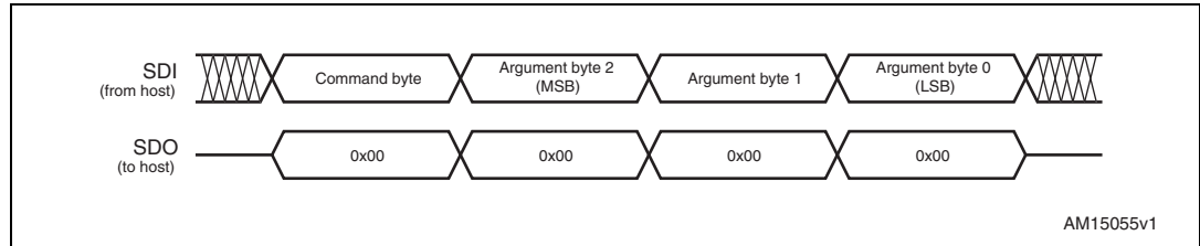
Figure 25. Command with 3-byte argument
