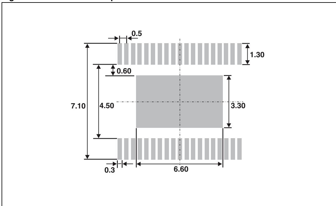
Figure 29. HTSSOP38 footprint
