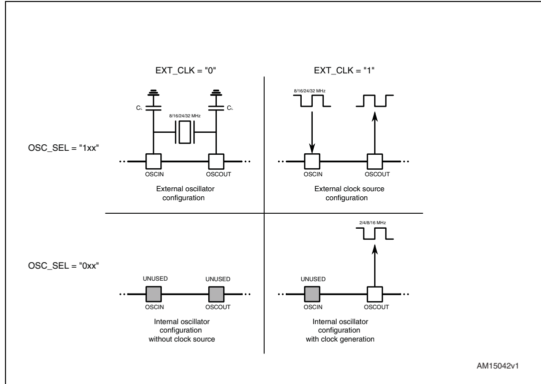
Figure 12. OSCIN and OSCOUT pin configuration
