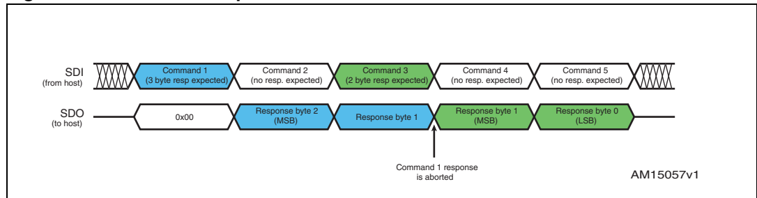
Figure 27. Command response aborted
