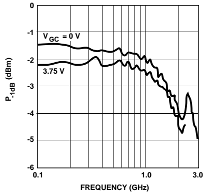
Figure 24. IVA-14208 P_{1dB} vs. Frequency and V_{GC} ; V_{CC} = 6\text{ V} , Frequency = 1\text{ GHz} , T_{case} = 25\text{ }^\circ\text{C} .
