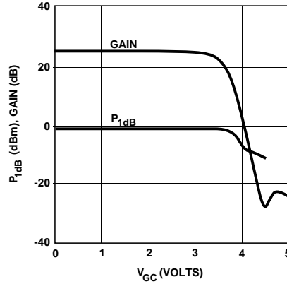
Figure 19. IVA-14208 Gain and P_{1dB} vs. V_{GC} ; V_{CC} = 6\text{ V} , Frequency = 1\text{ GHz} , T_{case} = 25\text{ }^\circ\text{C} .
