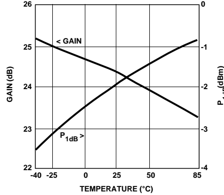
Figure 25. IVA-14208 Gain and P_{1dB} vs. Temperature; V_{CC} = 6\text{ V} , V_{GC} = 0\text{ V} , Frequency = 1\text{ GHz} .
