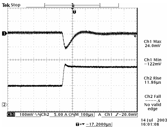
50% to 100% load Transient at Vin=5 V, Vo=1.2 V
