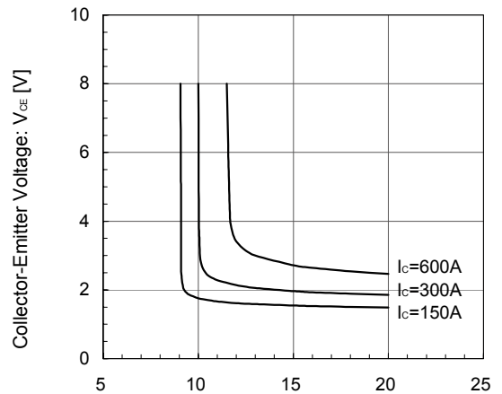
Collector-Emittter voltage vs. Gate-Emittter voltage (typ.) T_J = 25^\circ\text{C} / chip
