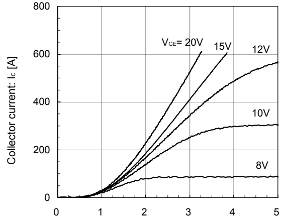
Collector current vs. Collector-Emittter voltage (typ.) T_J = 150^\circ\text{C} / chip
