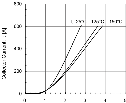
Collector current vs. Collector-Emittter voltage (typ.) V_{GE} = 15\text{V} / chip
