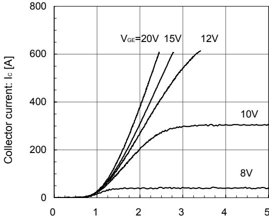
Collector current vs. Collector-Emittter voltage (typ.) T_J = 25^\circ\text{C} / chip
