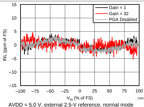
Figure 8. Integral Nonlinearity vs Differential Input Signal
