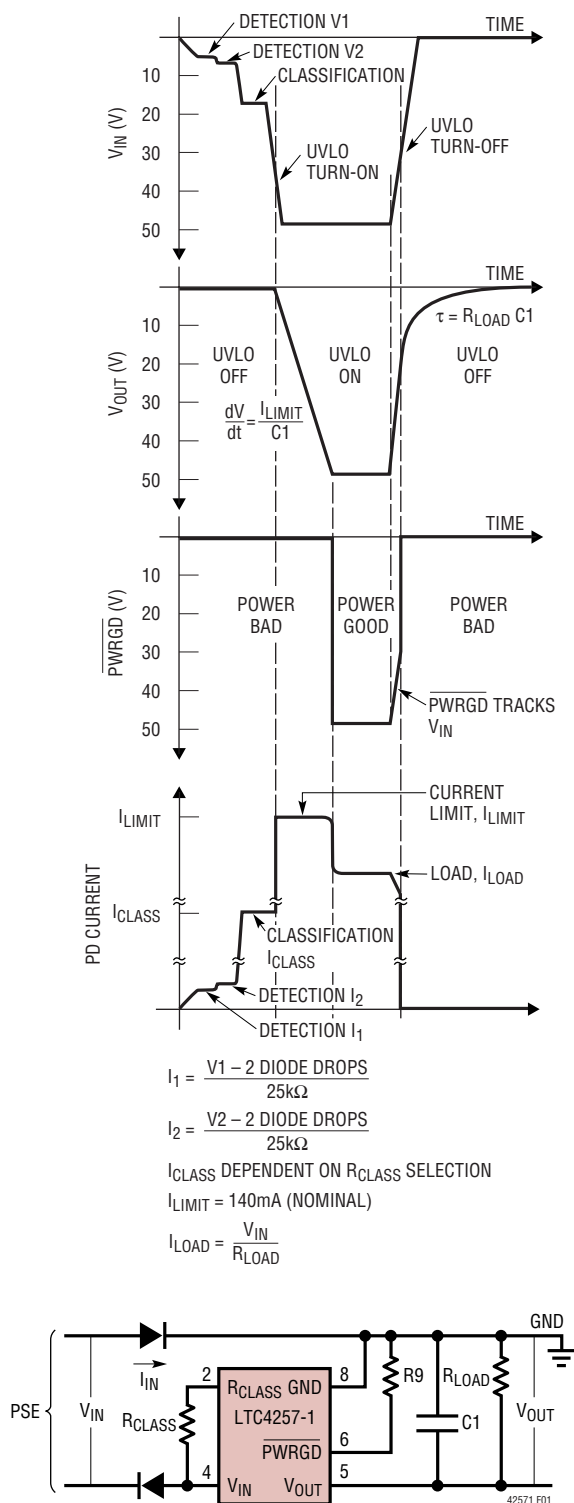
Figure 1. Output Voltage, \overline{\text{PWRGD}} and PD Current as a Function of Input Voltage
