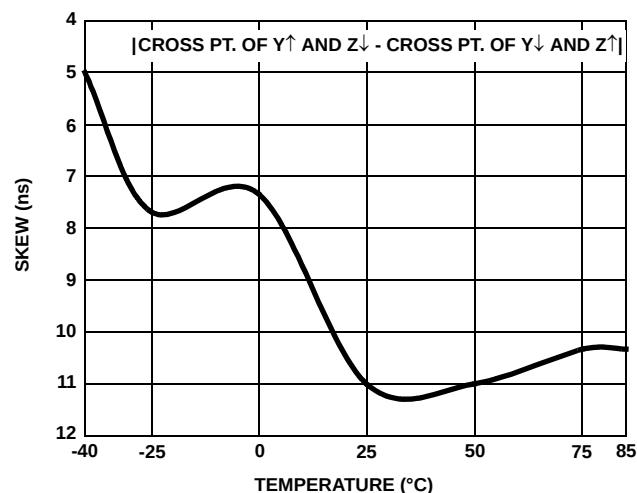
FIGURE 13. DRIVER DIFFERENTIAL SKEW vs TEMPERATURE (ISL3150E, ISL3152E)
