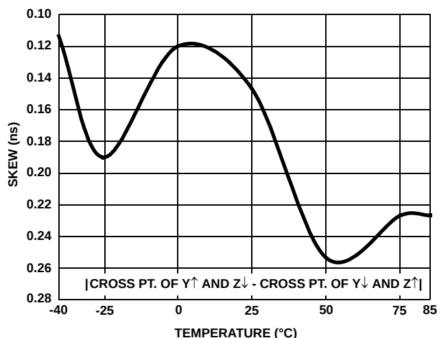
FIGURE 17. DRIVER DIFFERENTIAL SKEW vs TEMPERATURE (ISL3156E, ISL3158E)
