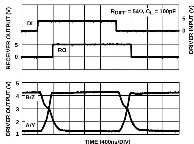
FIGURE 19. DRIVER AND RECEIVER WAVEFORMS, (ISL3153E, ISL3155E)
