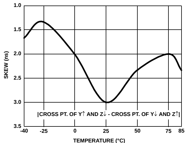
FIGURE 15. DRIVER DIFFERENTIAL SKEW vs TEMPERATURE (ISL3153E, ISL3155E)
