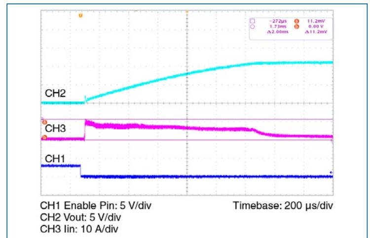
Figure 4 — Inrush current
