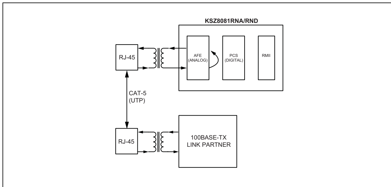
FIGURE 3-8: REMOTE (ANALOG) LOOPBACK
