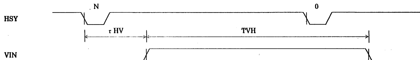
Fig.2-g Output signal timing of LOWO
