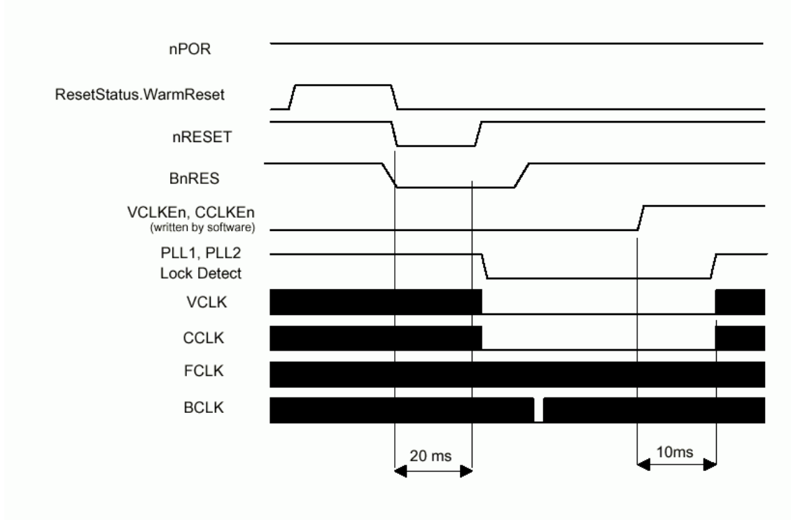
Figure 5-3 PMU Software Generated Warm Reset
