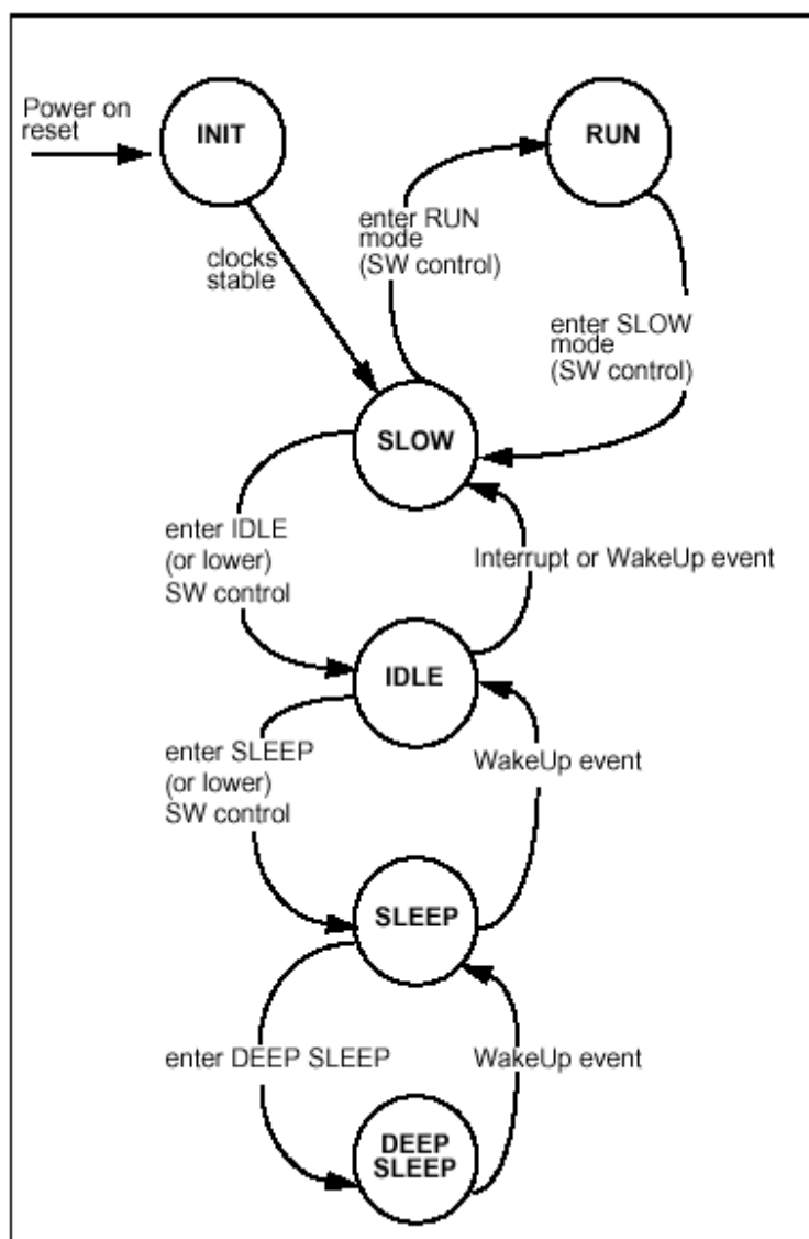
Figure 5-1 PMU Power Management State Diagram
