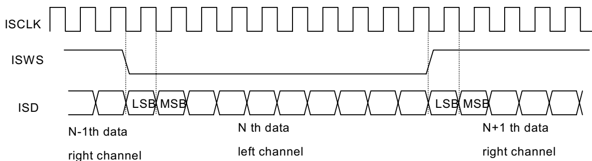
Figure 9-1 I²S Timing Diagram
