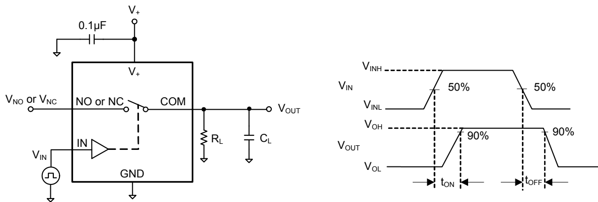
Test Circuit 2. Switching Times
