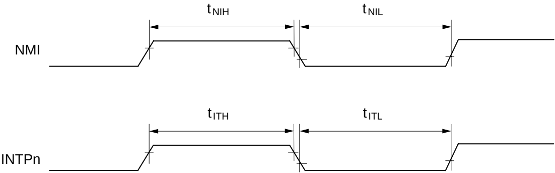
Figure 3-7: Interrupt Timing
