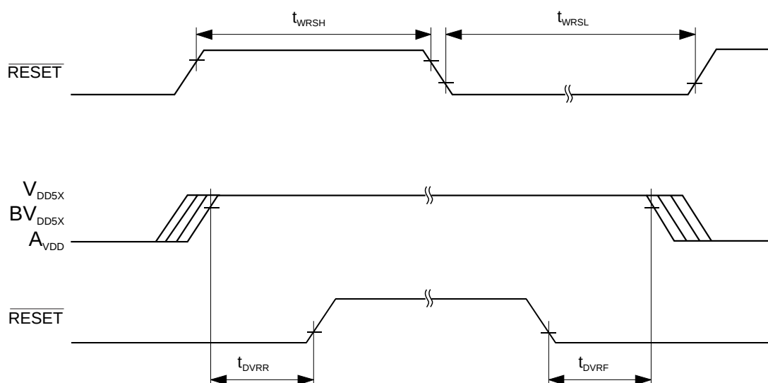
Figure 3-6: Reset Timing
