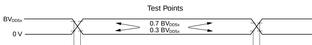
Figure 3-2: AC Test Input/Output Waveform
