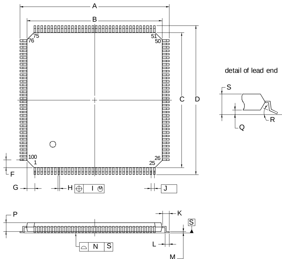
Figure 4-1: Package Drawing
