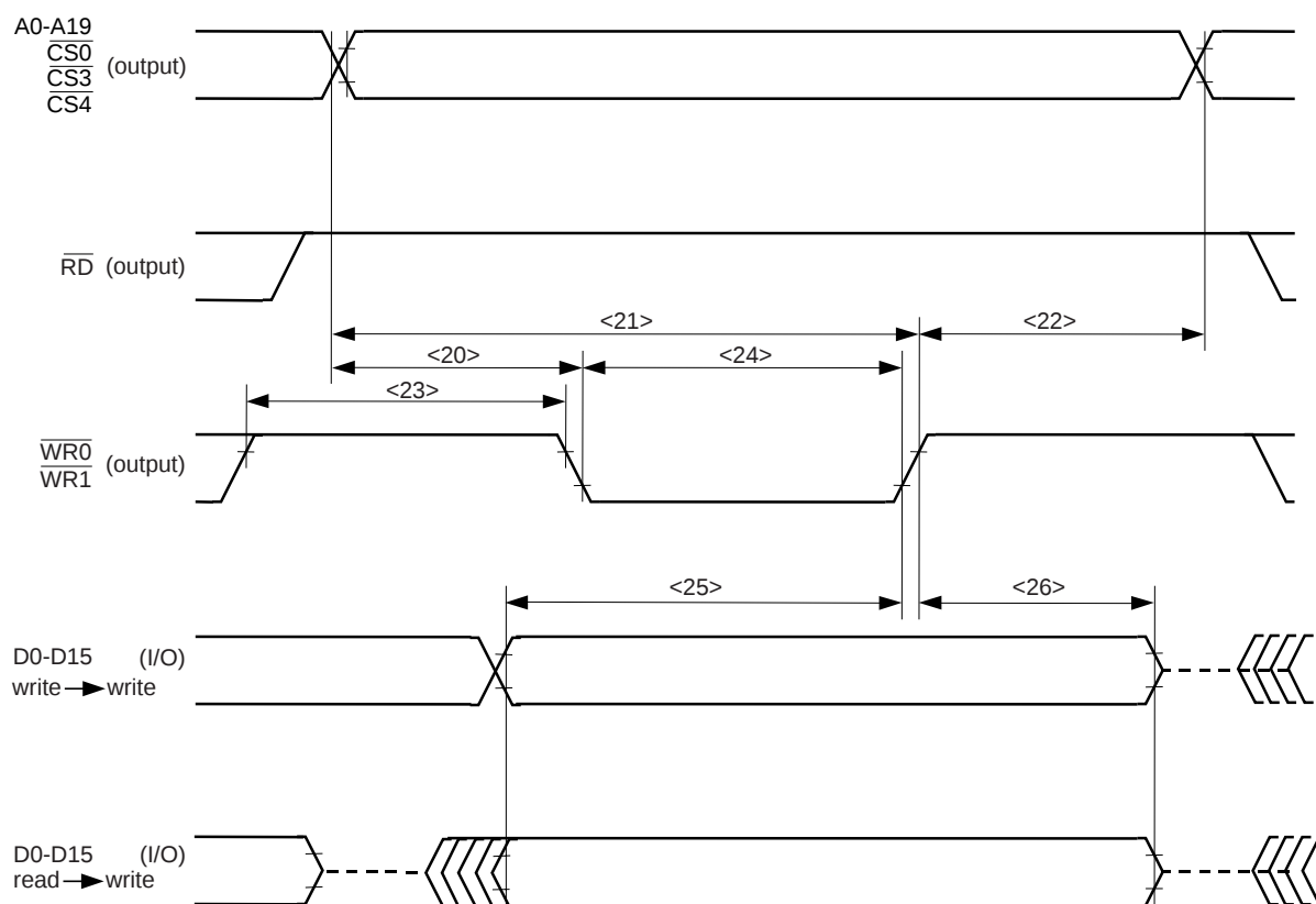
Figure 3-5: SRAM Write Timing
