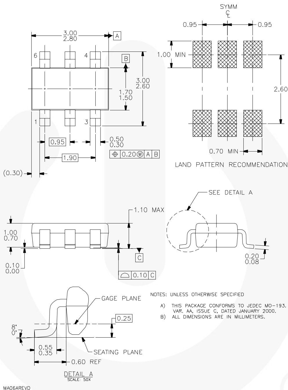
Figure 15. 6-Lead SUPERSOT6, JEDEC MO-193, 1.6mm Wide
