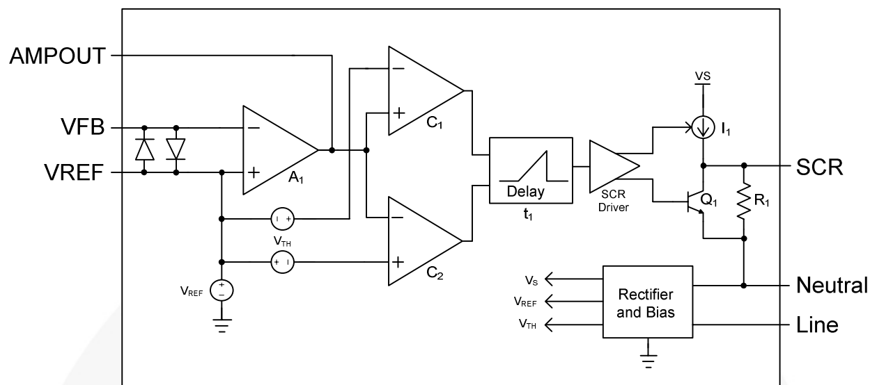
Figure 3. Block Diagram
