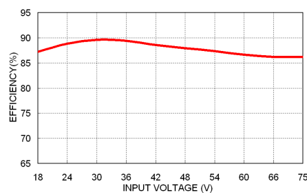
FKC12-48S05W Efficiency vs. Input Voltage
