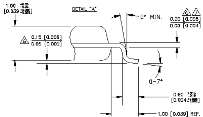
DETAIL VIEW
