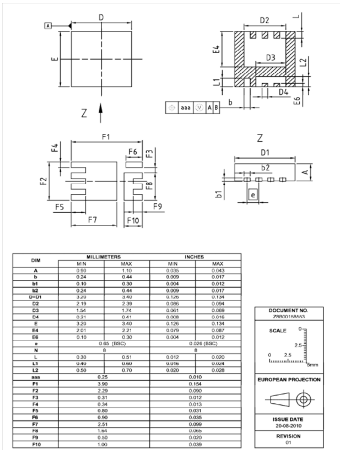
Figure 1 Outlines PG-TSDSON-8 ( fused leads ), dimensions in mm/inches
