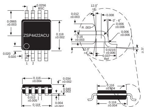
8-pin MSOP
