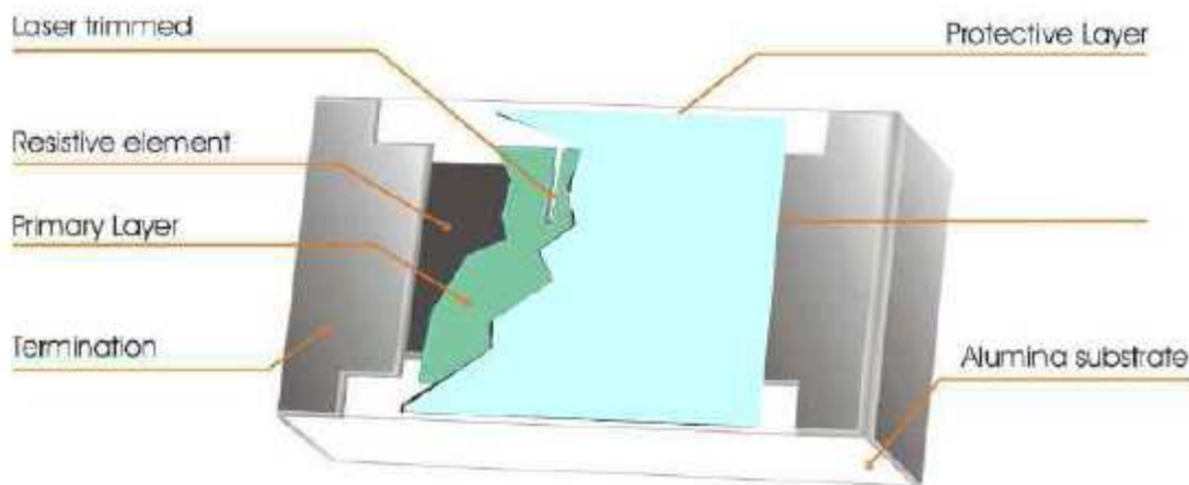
Fig 1. Construction of Chip-R
