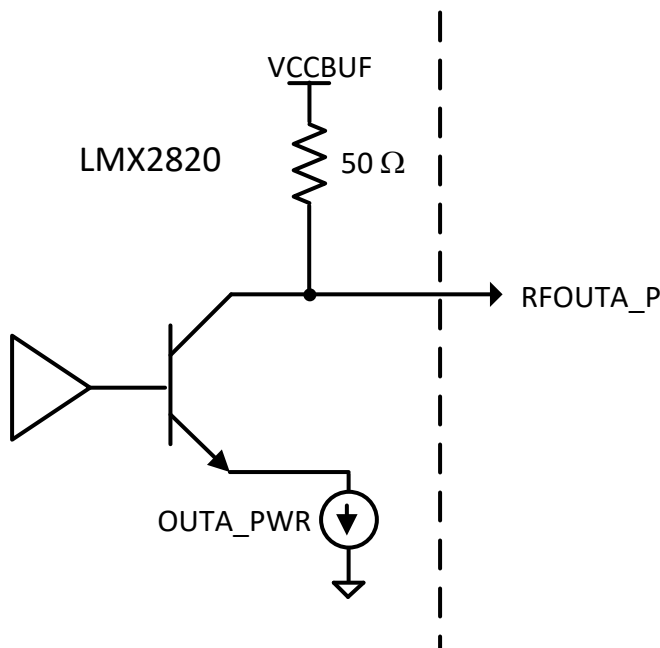
Figure 7-2. Output Buffer Structure
