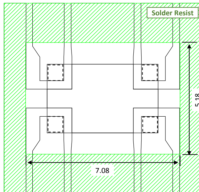
*Resist Pattern
