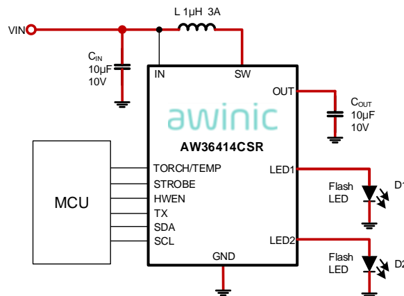
Fig 1 Typical Application Circuit of AW36414
