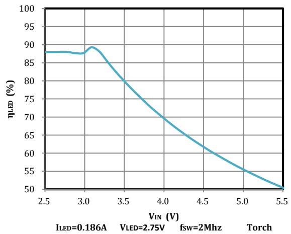
Fig28. LED Efficiency vs Input Voltage
