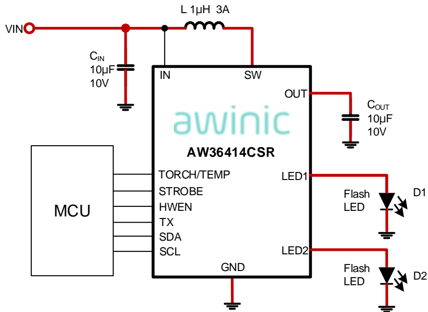
Fig 3 AW36414 Application Circuit
