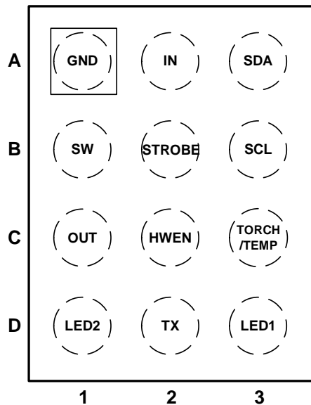
AW36414CSR Pin Configuration (Top View)
