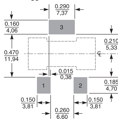
Suggested Land Pattern
