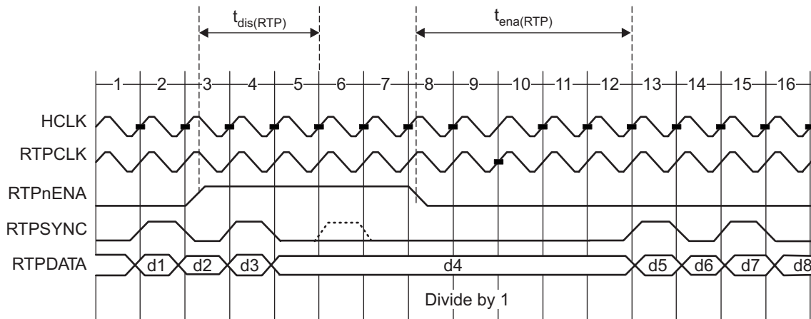
图 6-26. RTPnENA Timing
