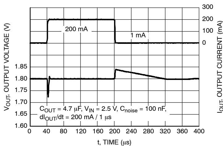
Figure 26. Load Transient Response, V_{OUT} = 1.8 V , C_{OUT} = 4.7 \mu F , C_{noise} = 100 nF
