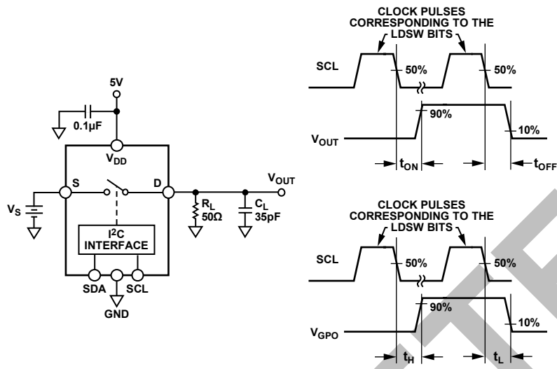
Figure 28. Switching Times
