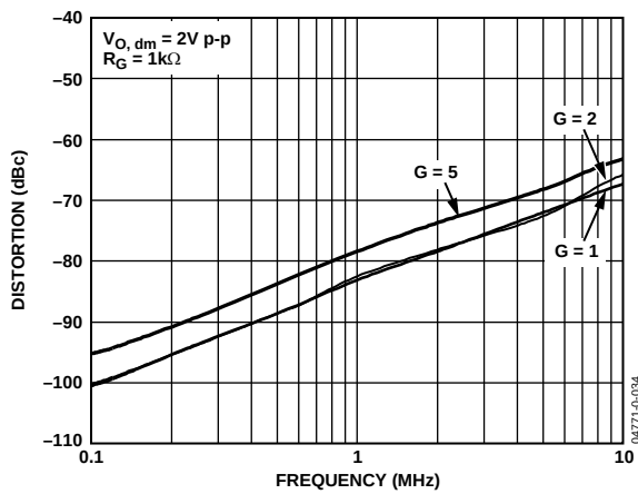
Figure 24. Second Harmonic Distortion at Various Gains
