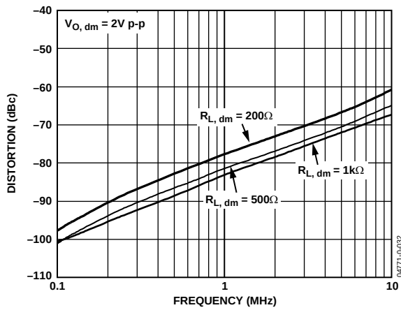
Figure 23. Second Harmonic Distortion at Various Loads
