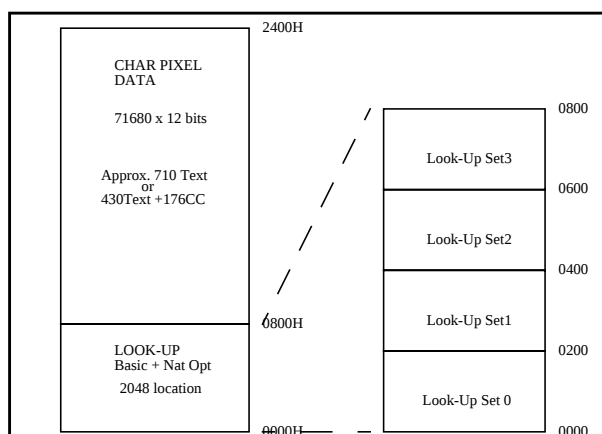
Fig.24 ROM Organisation
