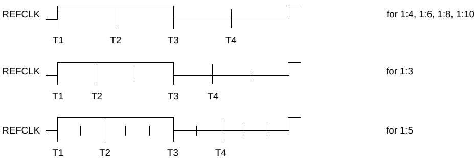
Figure 10. Internal Tick Spacing for Memory Controller Signals
