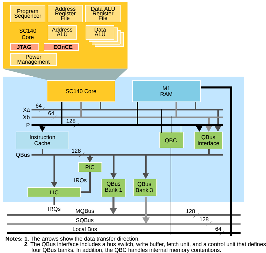
Figure 2. StarCore SC140 DSP Extended Core Block Diagram
