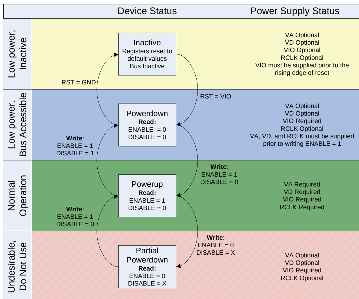
Figure 2. Powerup, Powerdown, and Reset State Diagram
