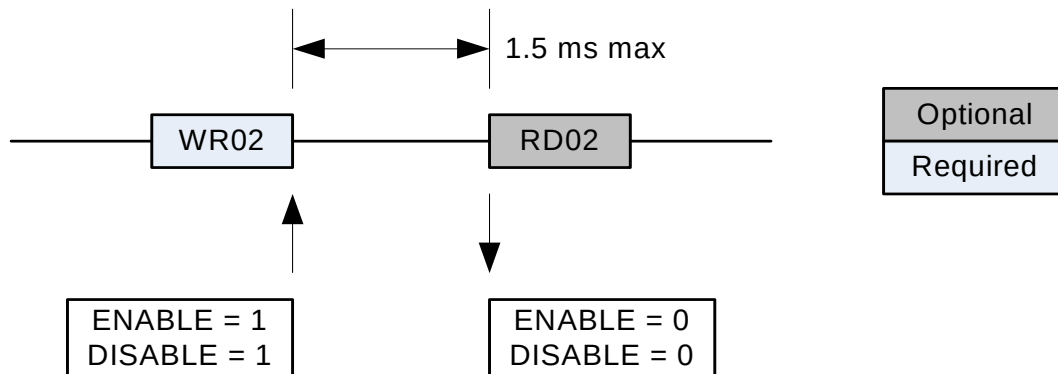
Figure 5. Powerdown Timing
