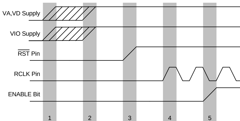
Figure 1. Initialization Sequence
