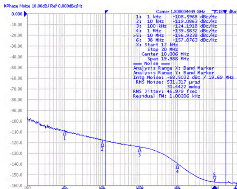
图 8-12. Typical Jitter
