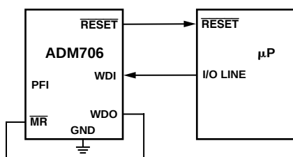
Figure 16. \overline{\text{RESET}} from WDO
