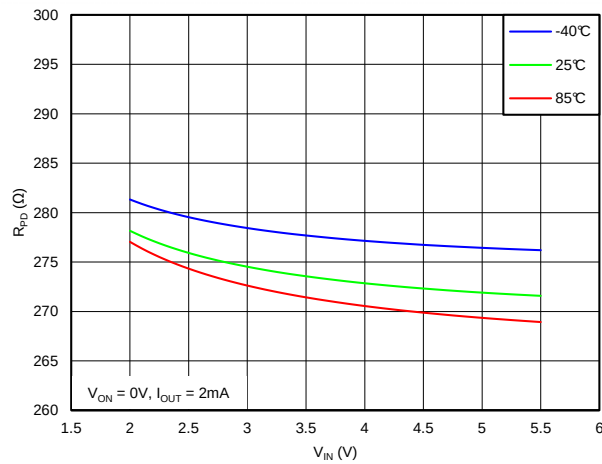
图 7. Output Pulldown Resistance vs V_{IN}
