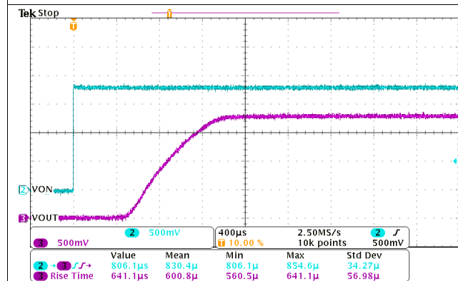
图 26. Turn-On Response Time ( V_{IN} = 2.5\text{ V} , C_{IN} = 1\text{ }\mu\text{F} , C_{OUT} = 0.1\text{ }\mu\text{F} , R_{OUT} = 10\text{ }\Omega )
