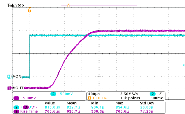
图 24. Turn-On Response Time ( V_{IN} = 3.3\text{ V} , C_{IN} = 1\text{ }\mu\text{F} , C_{OUT} = 0.1\text{ }\mu\text{F} , R_{OUT} = 10\text{ }\Omega )
