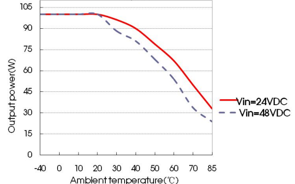
URF4812/15/24/48QB-100WFR3 Temperature Derating Curves
